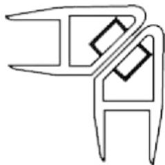
Code : 9272 Description : Glass to Glass 90° (Magnetic Seal) Application : 10 mm / 12 mm
