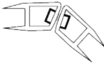
Code : 9273 Description : Glass to Glass 135° (Magnetic Seal) Application : 10 mm / 12 mm
